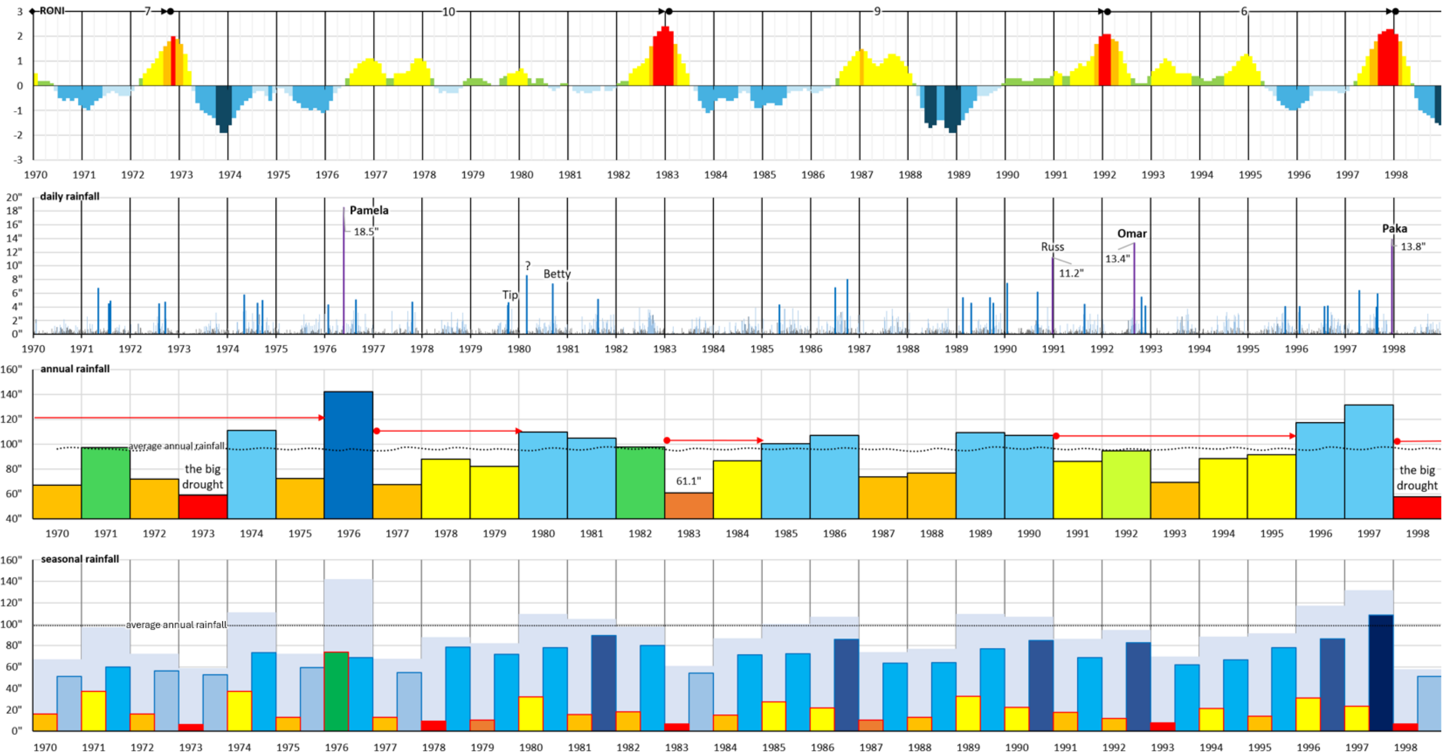
The Big Picture: ENSO RONI and Rainfall History (1970-2026) daily, annual, and seasonal (1970-1998...)
