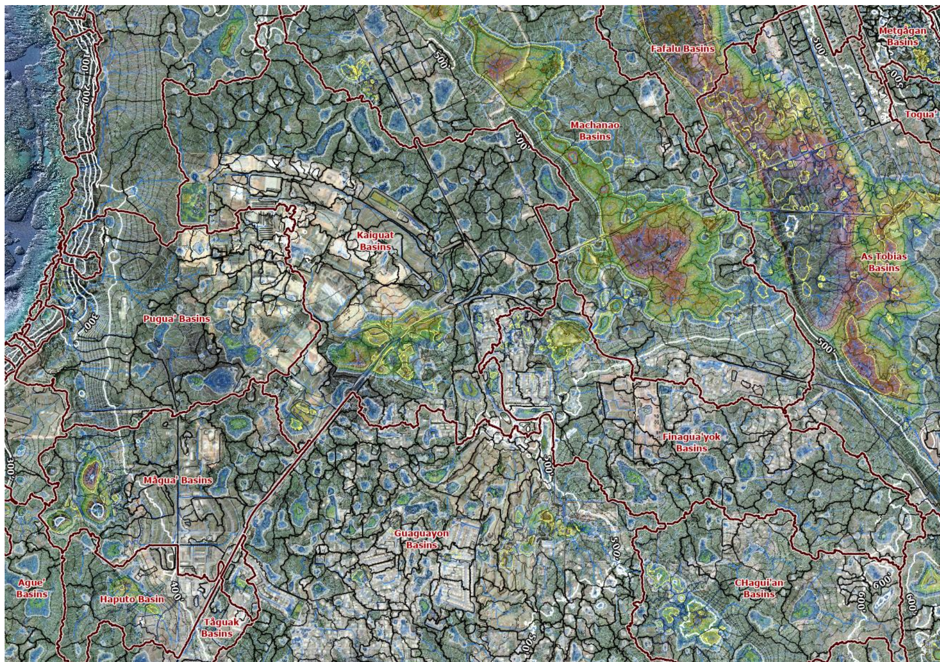
Northern Guam plateau basins surface hydrology analysis, soon to be added to the watershed map
