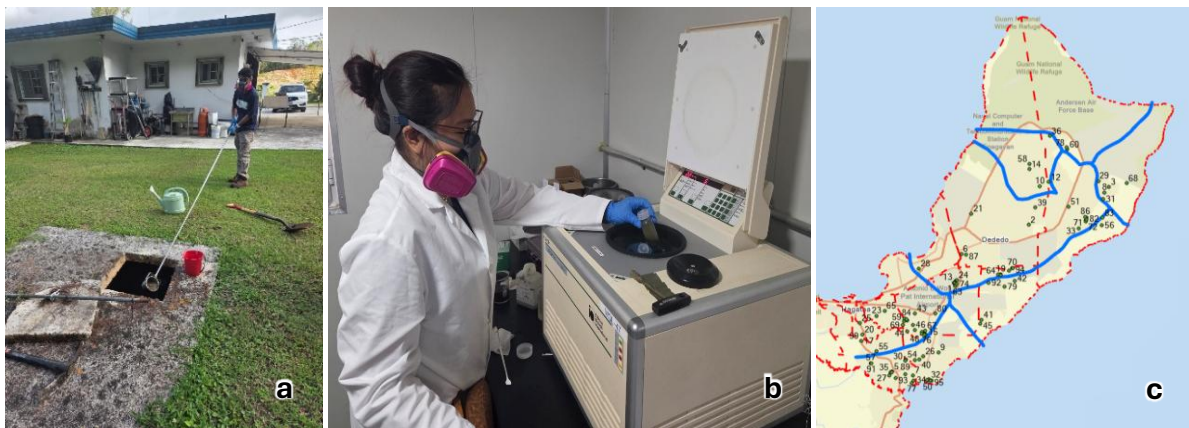
(a) Septic wastewater sampling, (b) Sludge separation process, and (c) GIS map of the sampling
