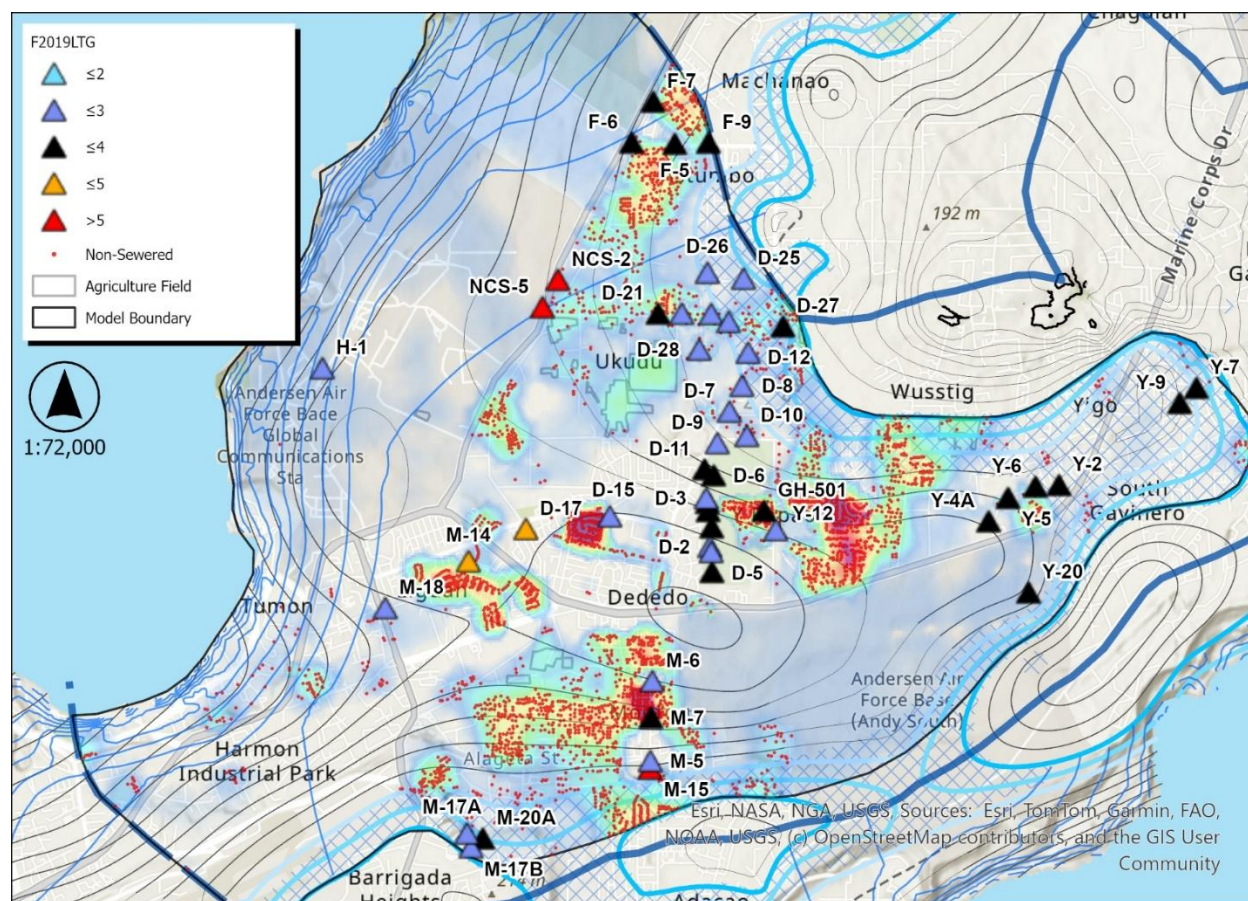
Model results show distinct nitrate plumes in areas with high septic system density across the Tomhom Aquifer Basin
