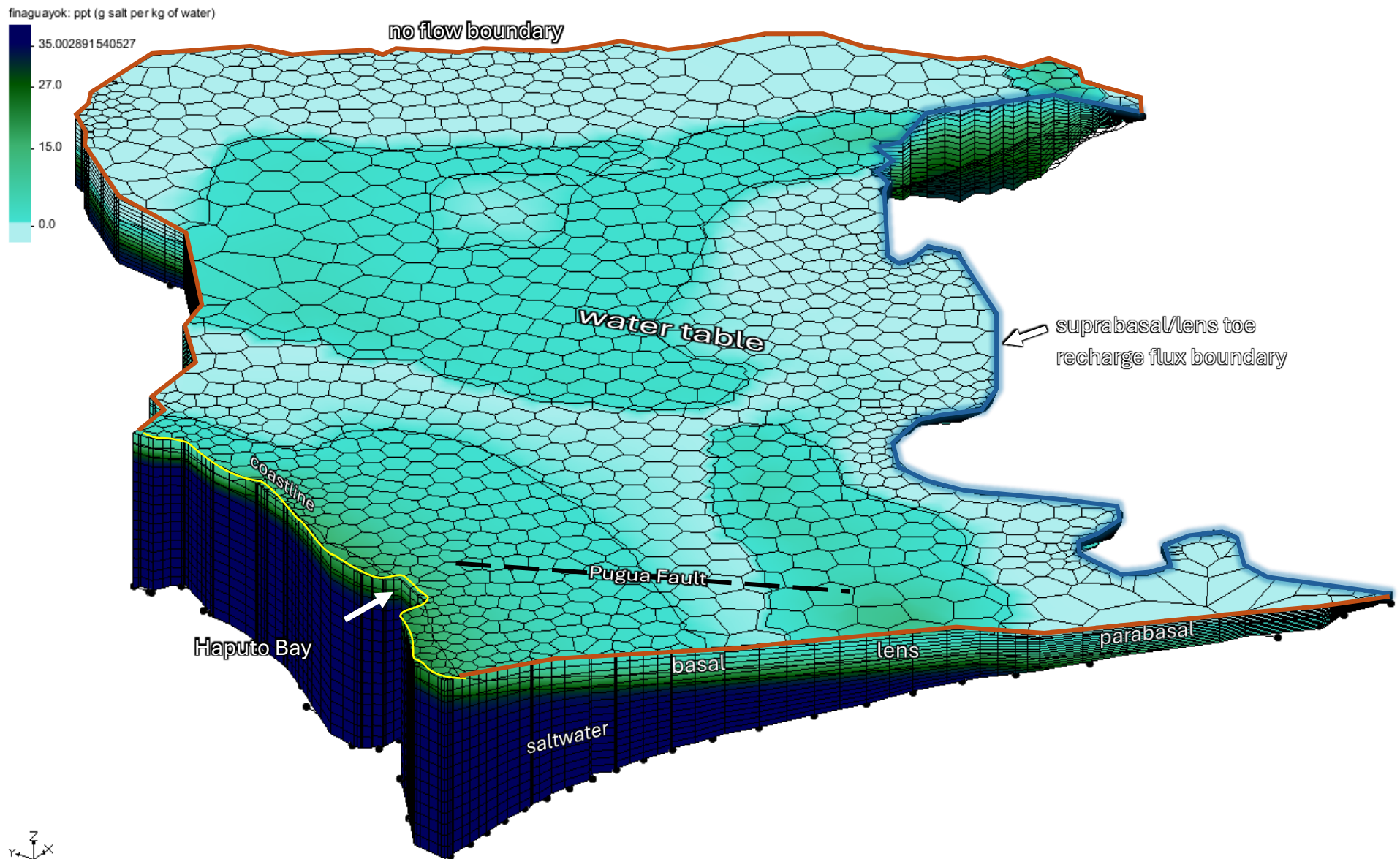
Finagua'yok Aquifer, phreatic groundwater flow model, Aquaveo GMS, MODFLOW-USG
