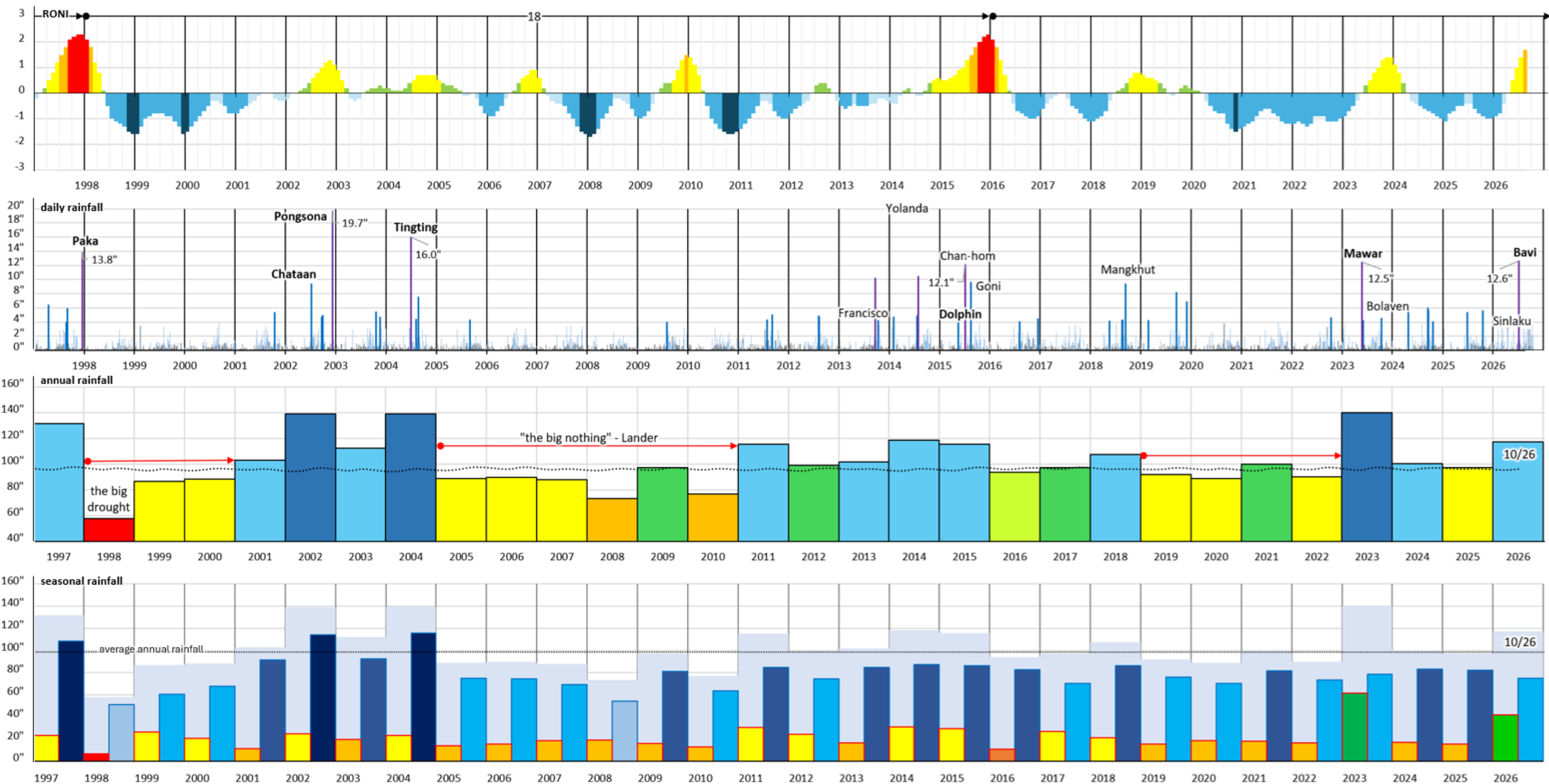
Continued... ENSO RONI and Rainfall History (1970-2026) daily, annual, and seasonal (...1997-10/18/2026)
