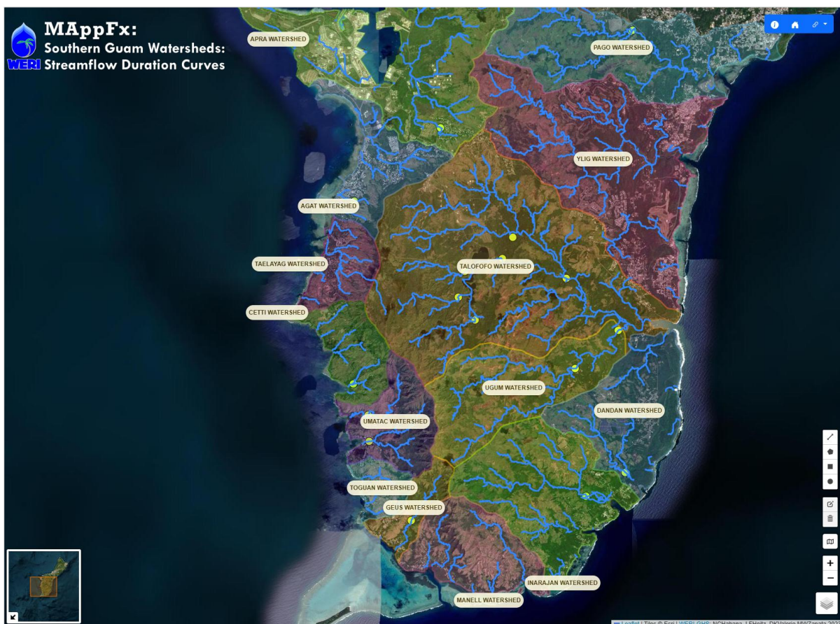
MAppFx: Southern Guam Watersheds: Streamflow Duration Curves
