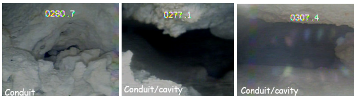
Screenshots from well D-18 (good water production)
