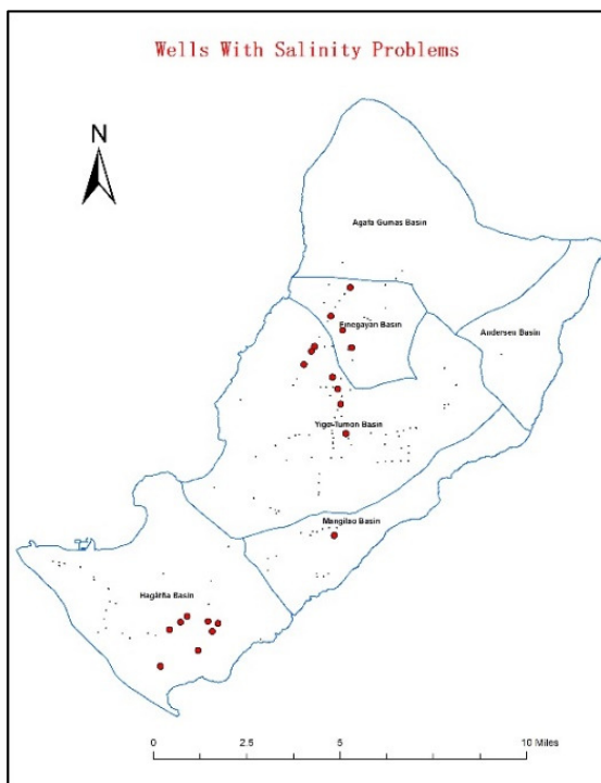
Wells with Salinity Problems
