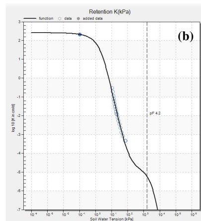
Experimental points and predicted curves for (a) SWRC and (b) unsaturated permeability for top soil
