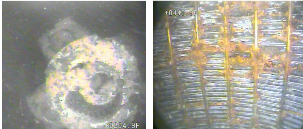
Pump stock (well A-9) and rusty well screen (well A-25)
