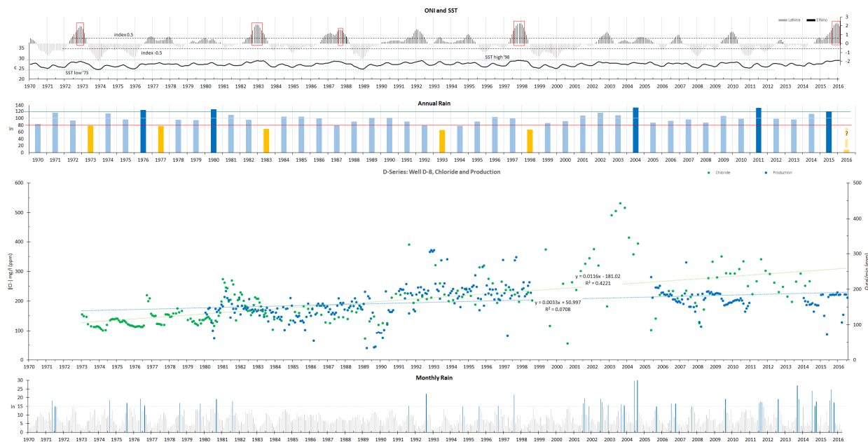
Rain, ONI and SST, chloride and production trend analysis, production well D-8.
