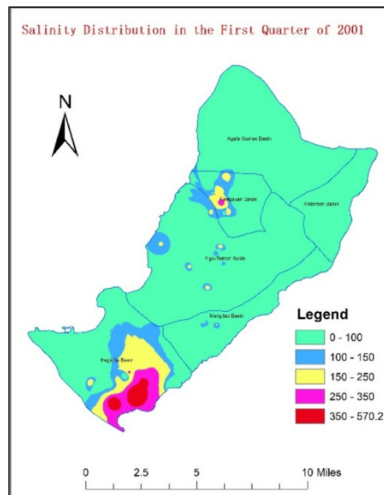
Salinity Distribution
