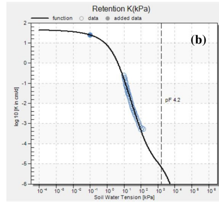
Experimental points and predicted curves for (a) SWRC and (b) unsaturated permeability for bottom soil
