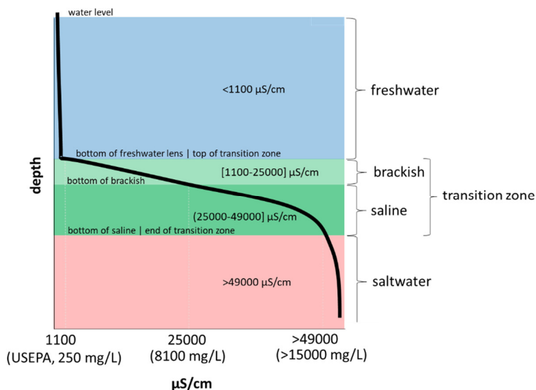
Salinity profile through the NGLA water layers.
