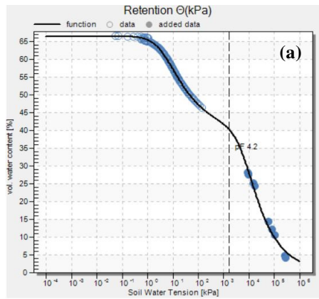
Experimental points and predicted curves for (a) SWRC and (b) unsaturated permeability for bottom soil
