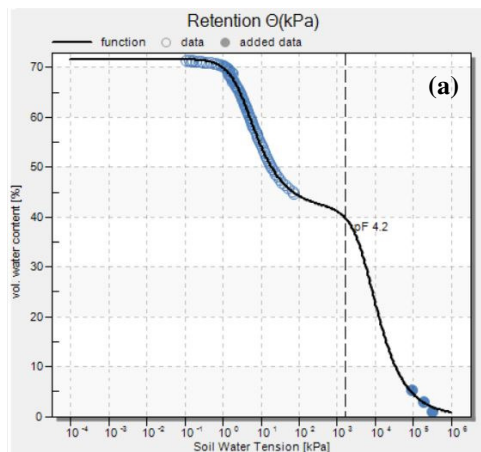
Experimental points and predicted curves for (a) SWRC and (b) unsaturated permeability for top soil
