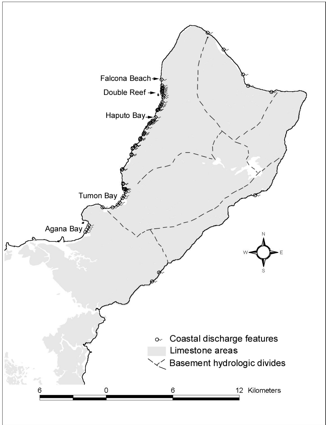
Fig. 15. Coastal discharge features in northern Guam. Also shown are the boundaries of the groundwater catchments that are defined by the ridges of the relatively impermeable basement rock.
