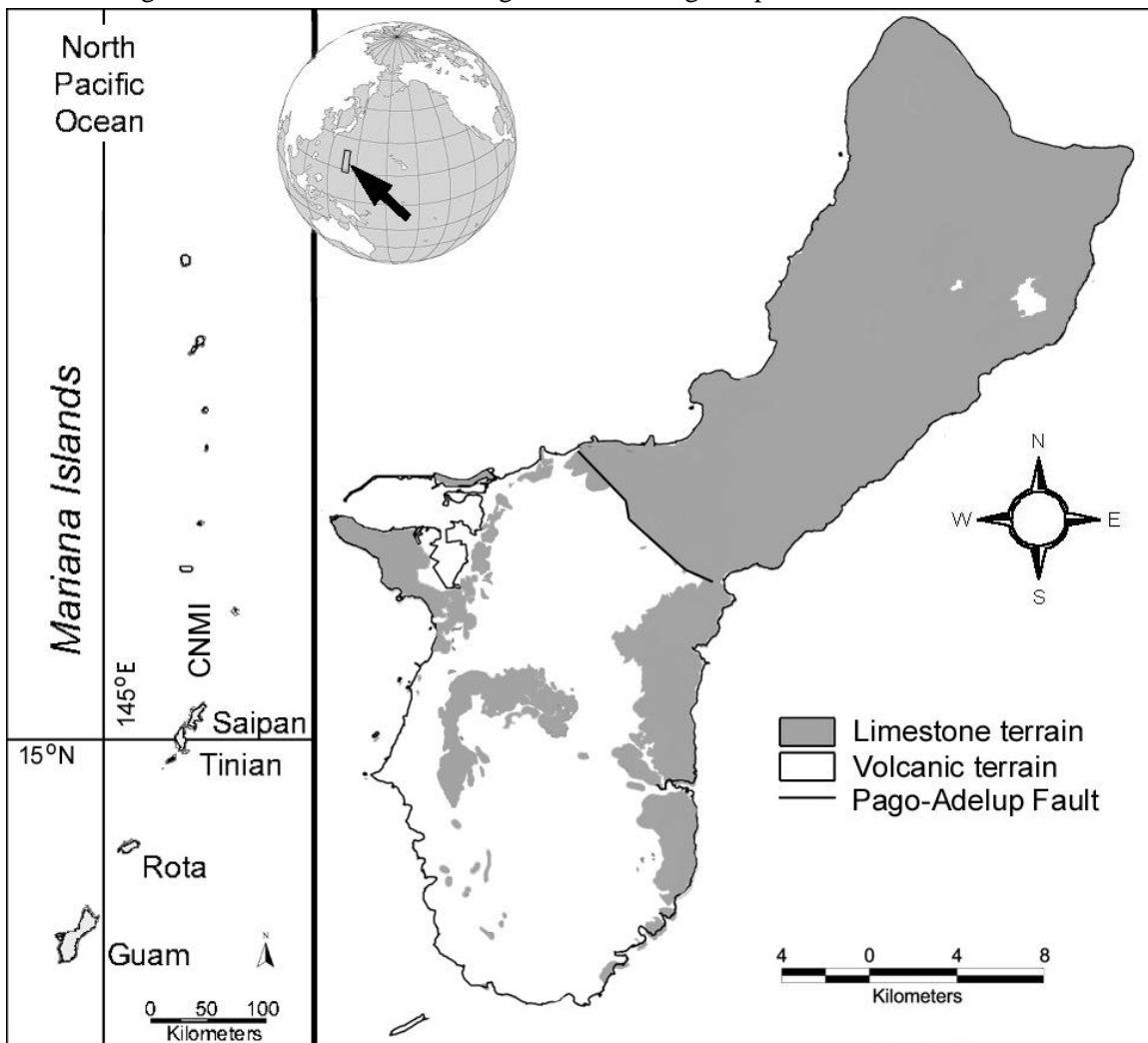
Fig. 1. Location of Guam and the extent of its limestone terrain over the two provinces separated by the Pago-Adelup Fault.
