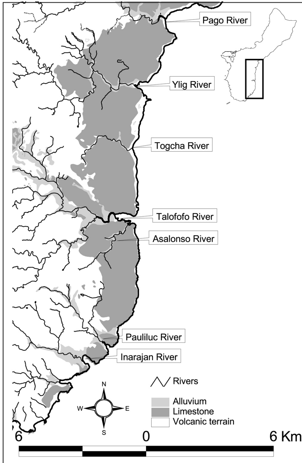
Fig. 10. Limestone coast of southern Guam.
