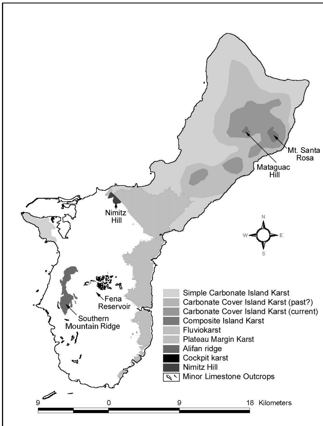
Fig. 4b. Karst environments of Guam. The north is almost entirely karst, with minor inliers of volcanic terrain at Mt. Santa Rosa and Mataguac Hill. The south is mostly volcanic terrain with karst on some outlying limestone units. The volcanic units also contain scattered minor outcrops of limestone.
