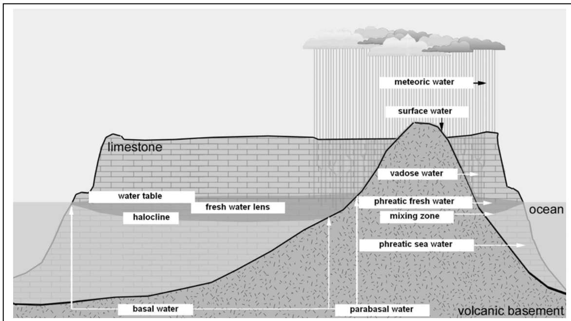
Fig. 3. Schematic cross-section of the Northern Guam Lens Aquifer. Not to scale.
