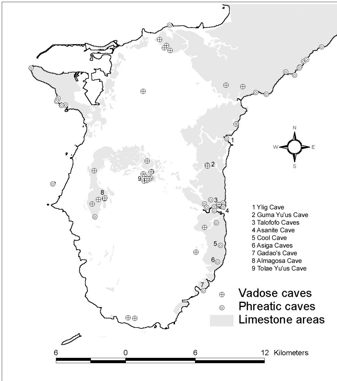
Fig. 14. Caves in southern Guam.
