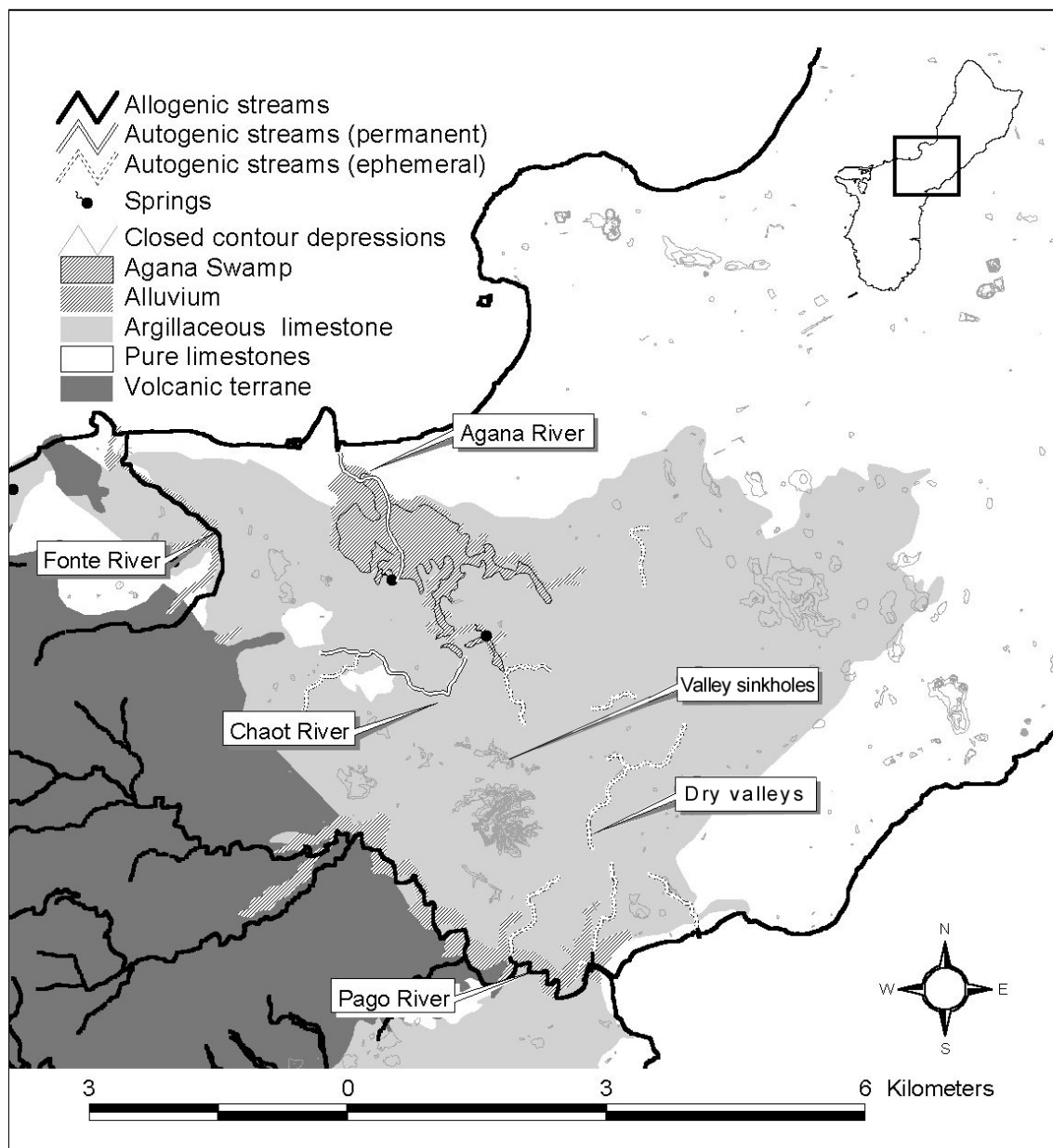
Fig. 5. Fluviokarst in the southern part of the northern Guam plateau.
