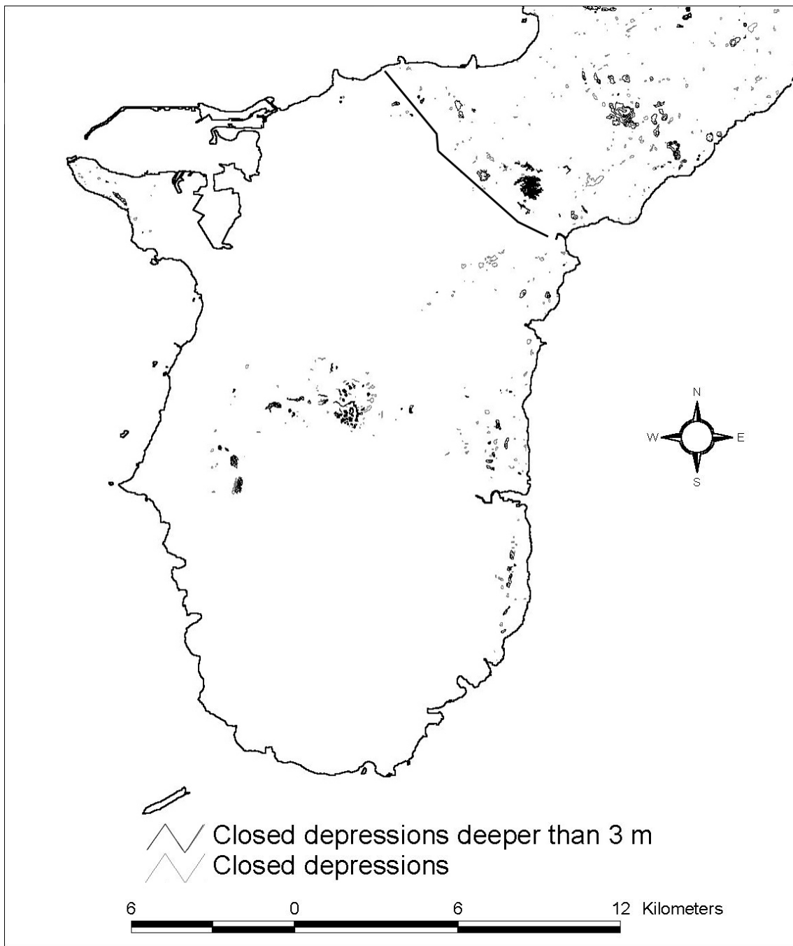
Fig. 12. Closed depressions in southern Guam.
