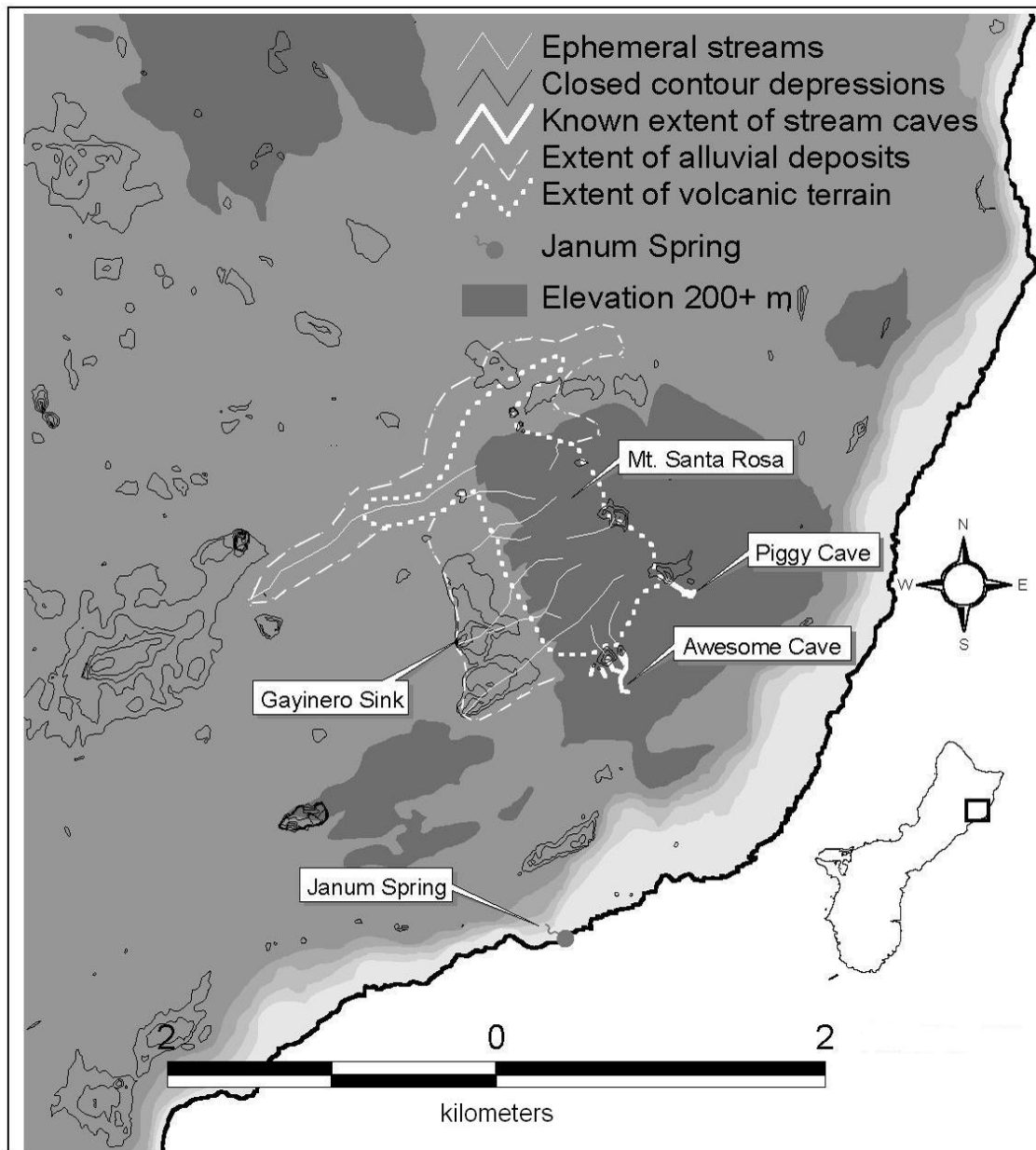
Fig. 7. Mt. Santa Rosa and associated karst features.
