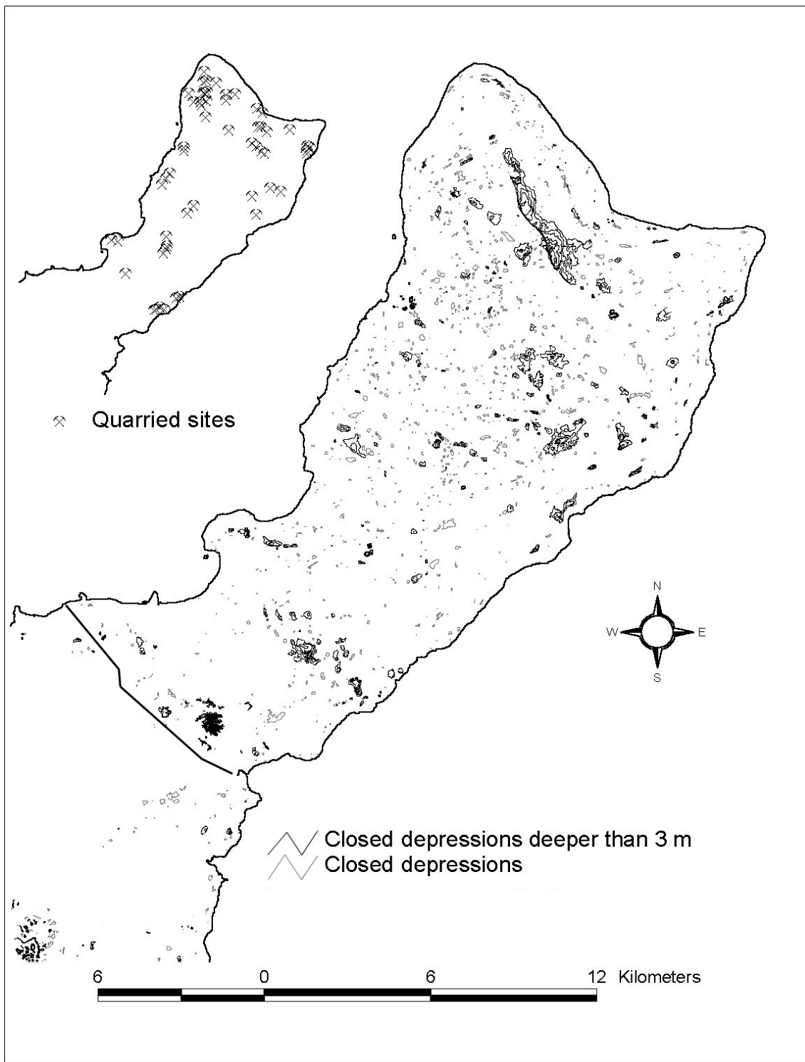
Fig. 11. Closed depressions in northern Guam, with inset showing quarried sites in northern Guam.
