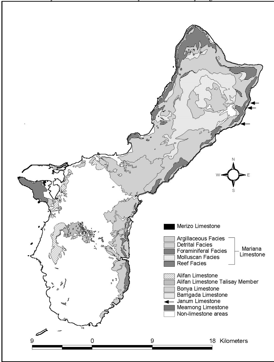
Fig. 2. Simplified geologic map showing the limestone units of Guam, based on Tracey et al. (1964).
