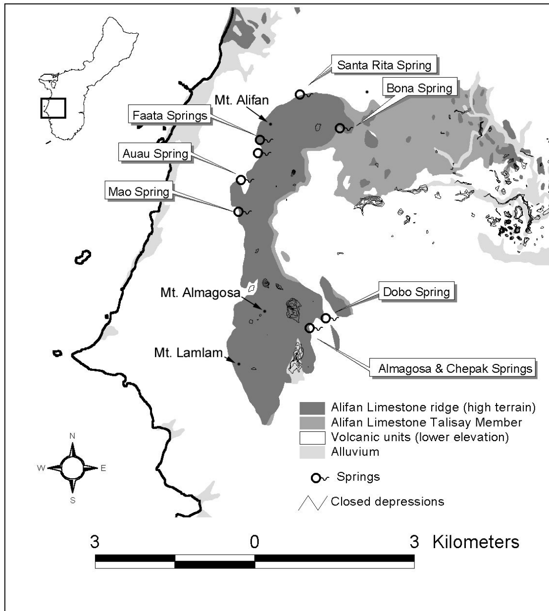
Fig. 8. Southern Mountain ridge and associated karst features.
