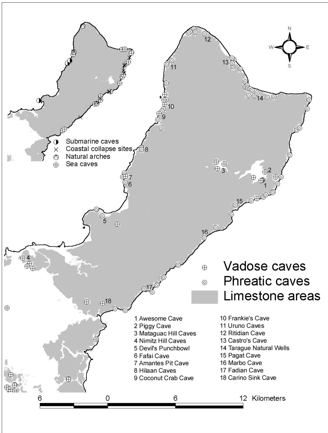
Fig. 13. Caves in northern Guam, with inset showing submarine caves, coastal cliff collapse sites, natural arches, and sea caves in northern Guam.
