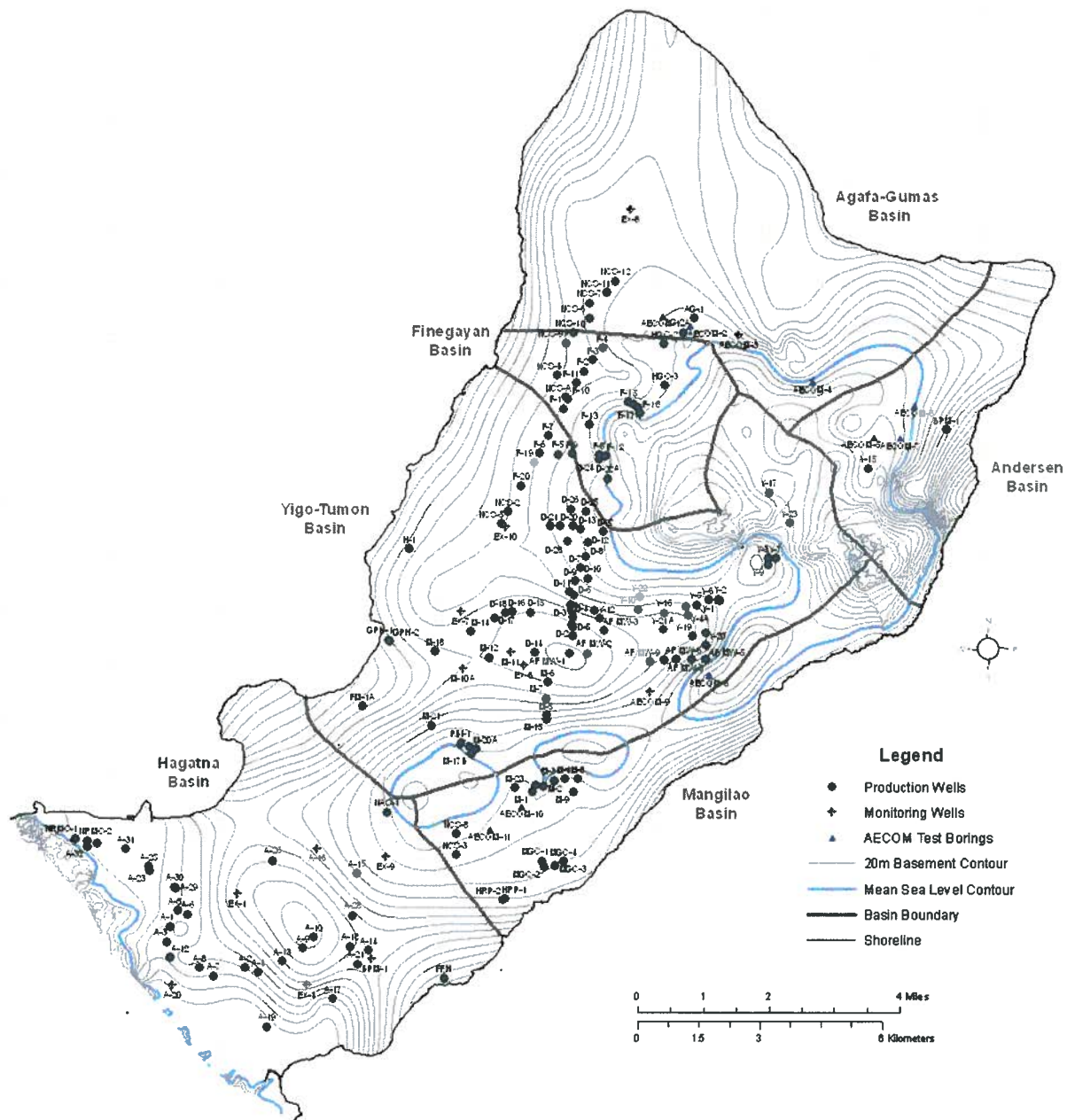
Figure 3: Volcanic basement contour map, with production and monitoring wells. (From Vann et al. 2014.)
