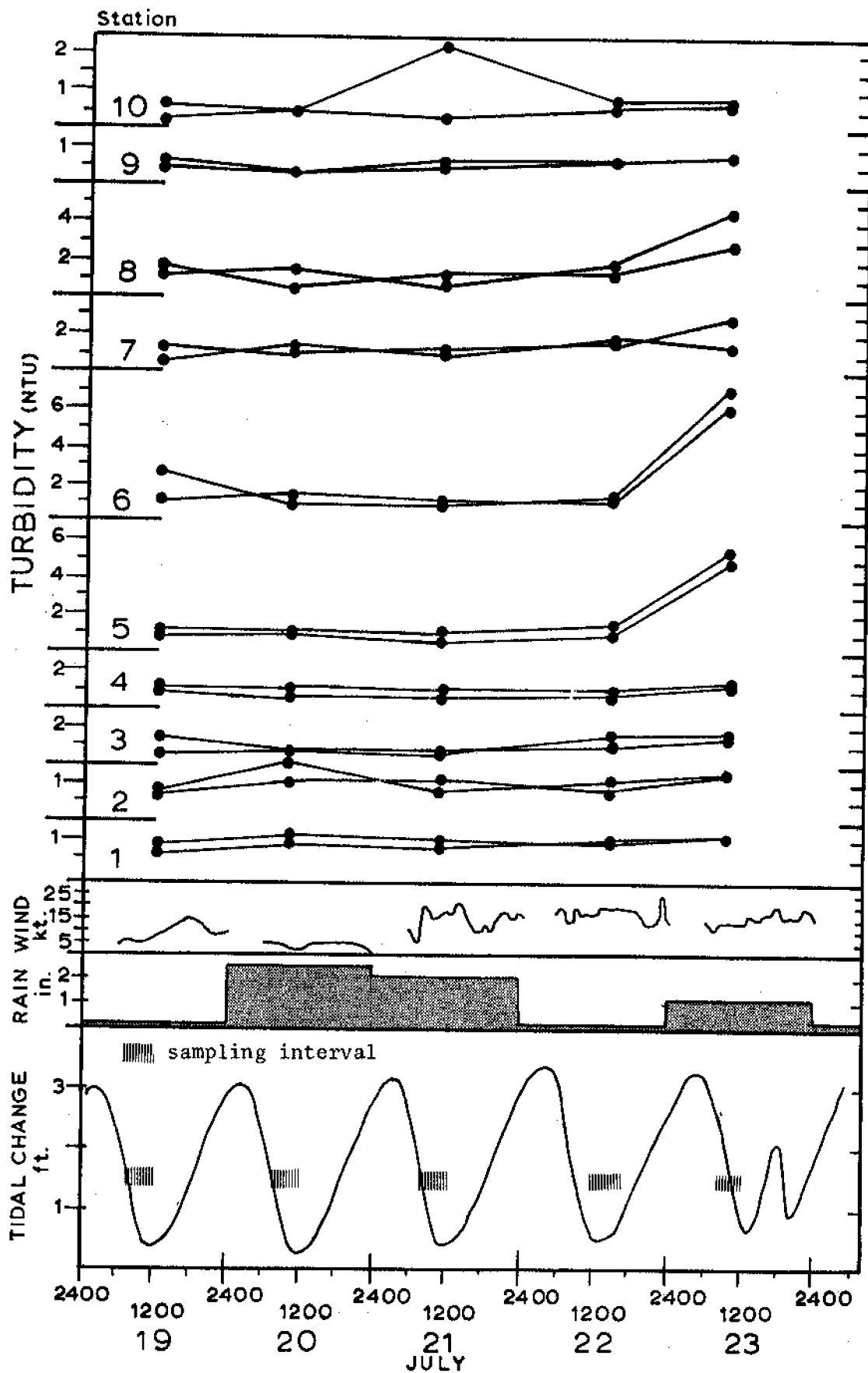
Figure 2. Monitoring station turbidities compared with meteorological conditions.
