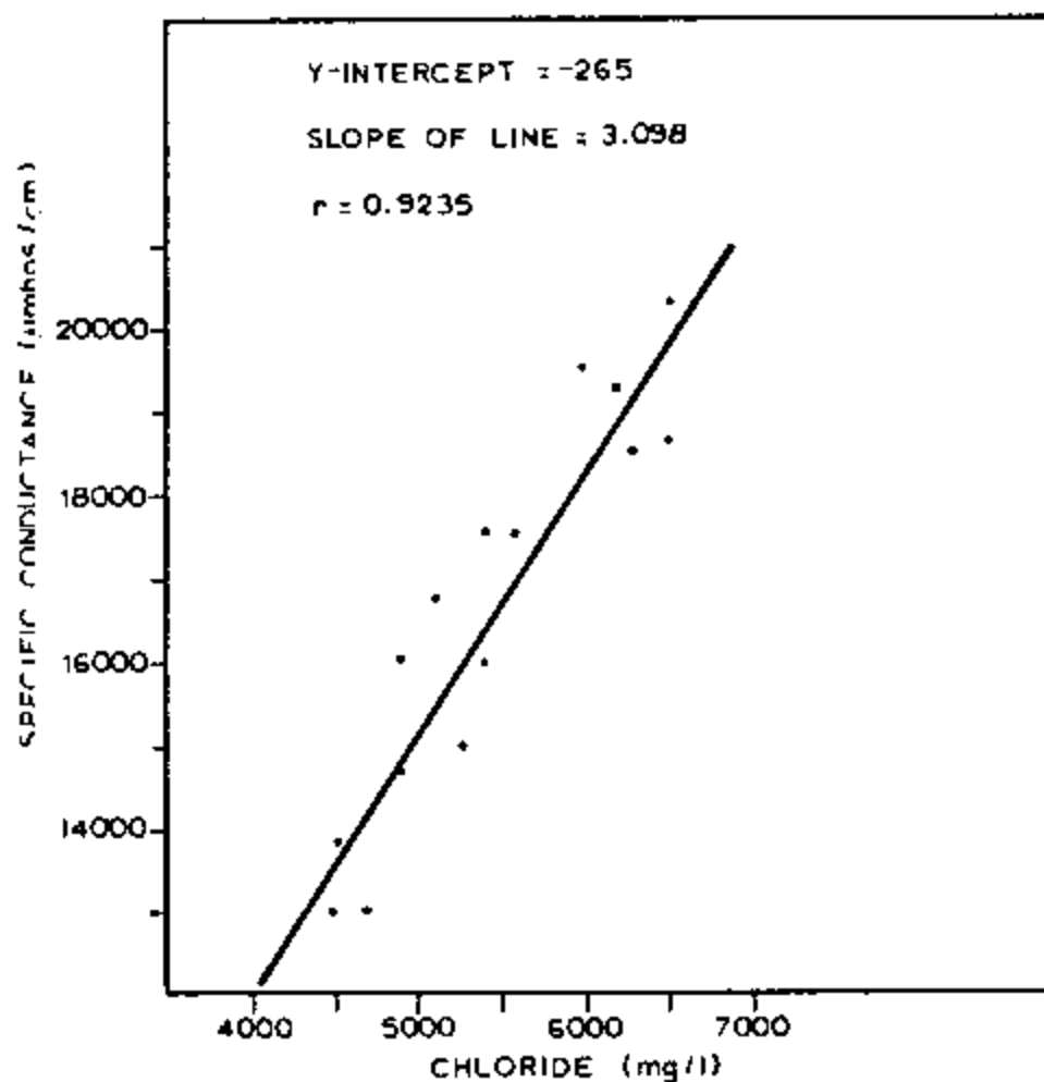
Figure D1. Calibration curve of specific conductance vs. chloride-ion concentration. Curve is used for \text{Cl}^- determination in collected water samples and borehole conductance measurements.
